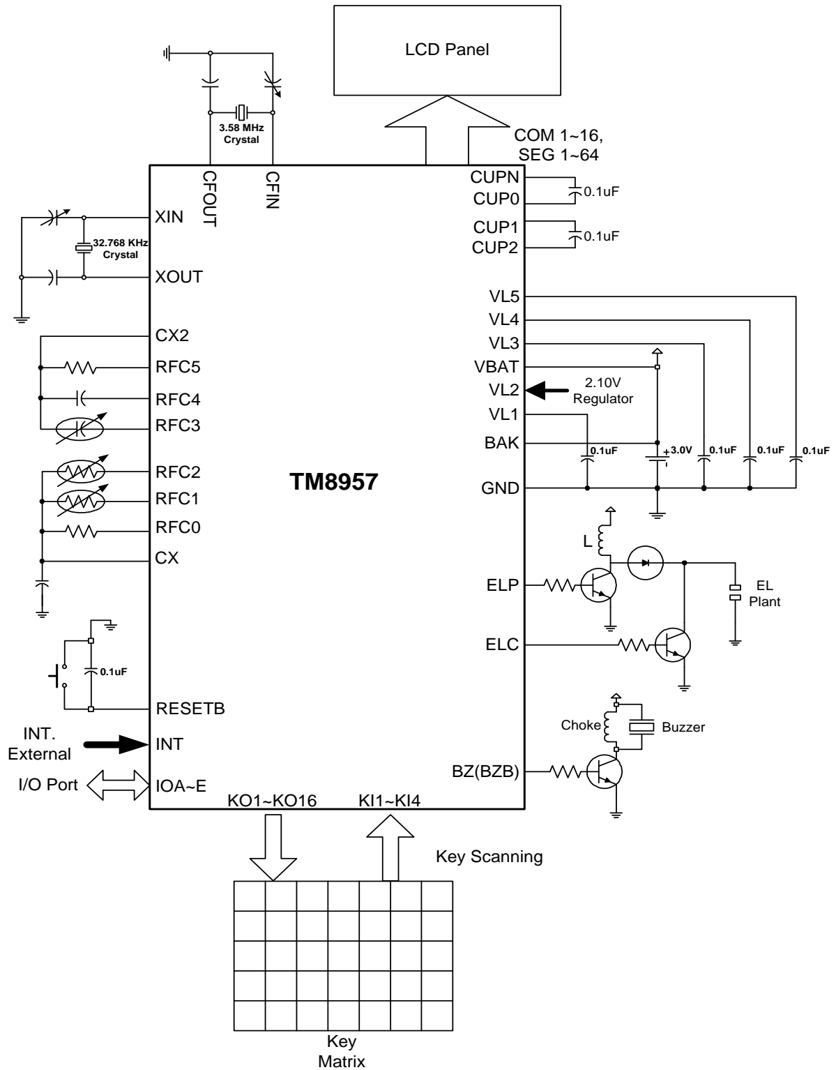
3V power mode (BAK = VBAT for BCF = 0), 1/5 Bias, 1/16 Duty
