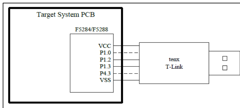
Figure 2-1. T-Link-EV5284/5288 Board
