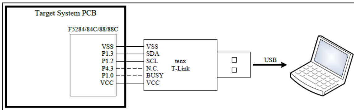
Figure 2-1. T-Link-EV5284/5288 Board
