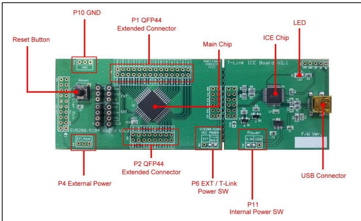
Figure 2-1. T-Link-EV5284/5288 Board
